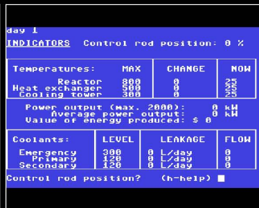
Nuclear Reactor
