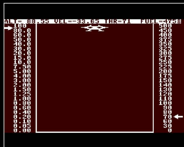
Lunar Lander
